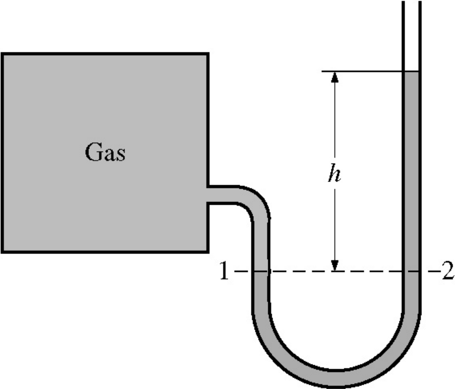
FIGURE 1-57 The basic manometer.
