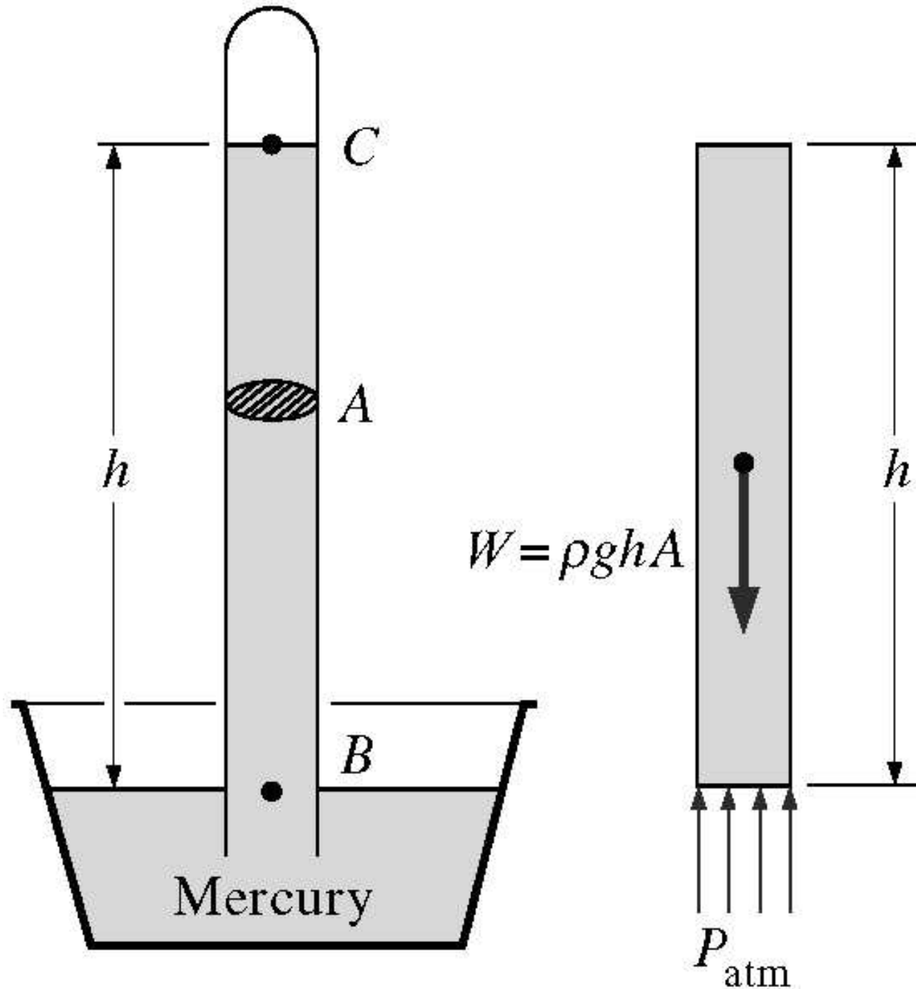
FIGURE 1-63 The basic barometer.
